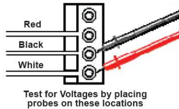
Figure 2. Proper Voltage Readings Across Terminals on House Breaker Box, Spa System Box and GFCI
