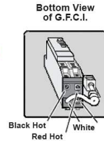
Figure 2. Proper Voltage Readings Across Terminals on House Breaker Box, Spa System Box and GFCI
