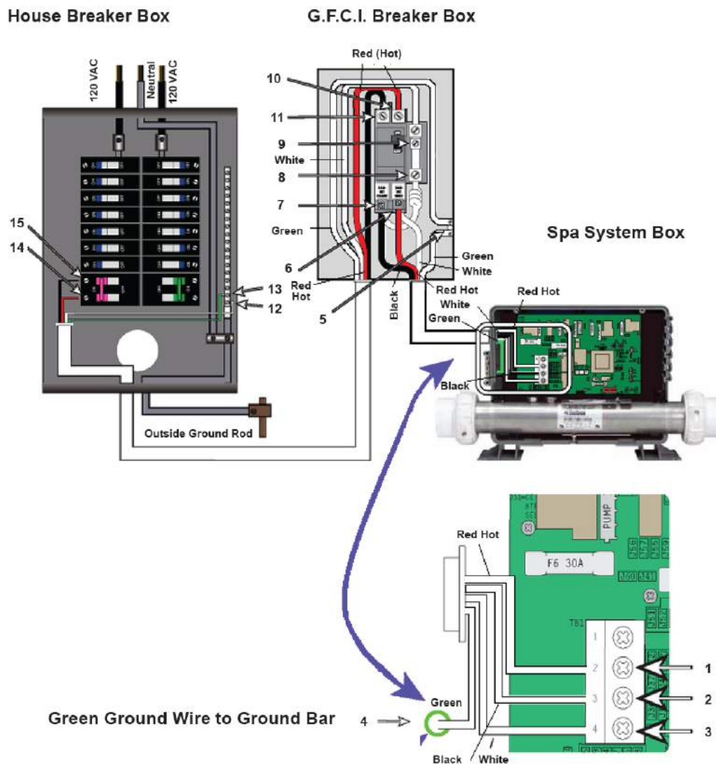
Figure 1. GFCI Wiring Schematic for 60 Hz Systems
