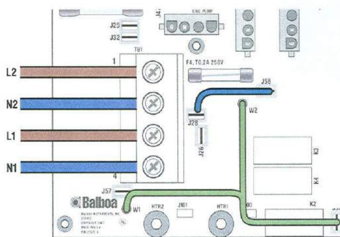
Figure 5. Two Phase Power – TN and TT Electrical Systems
