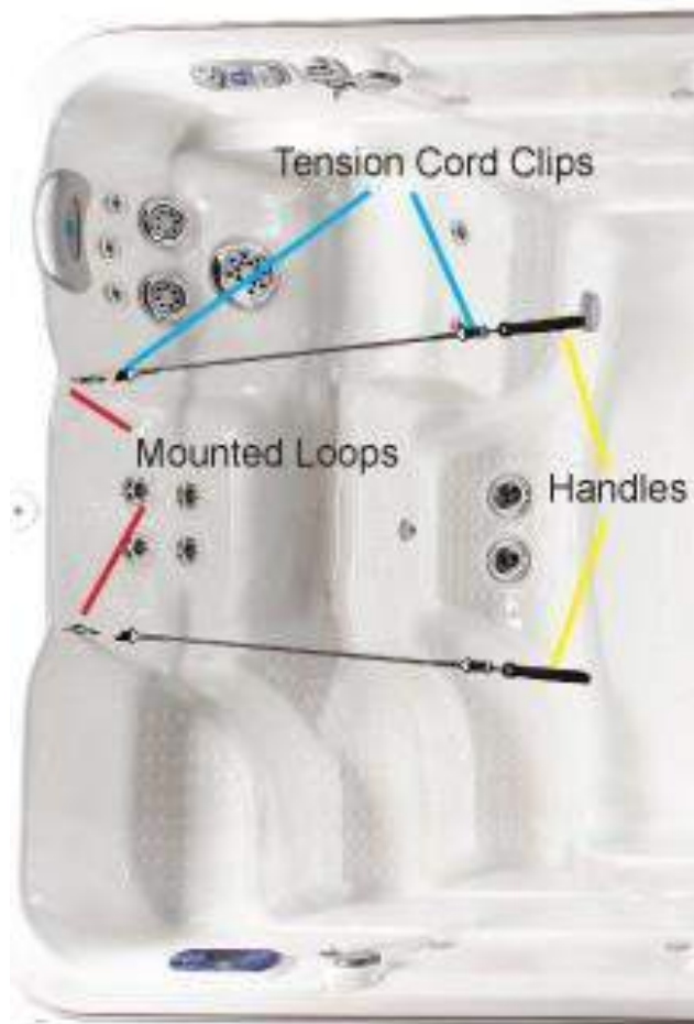
Figure 12. Tension Cord Mount Locations
