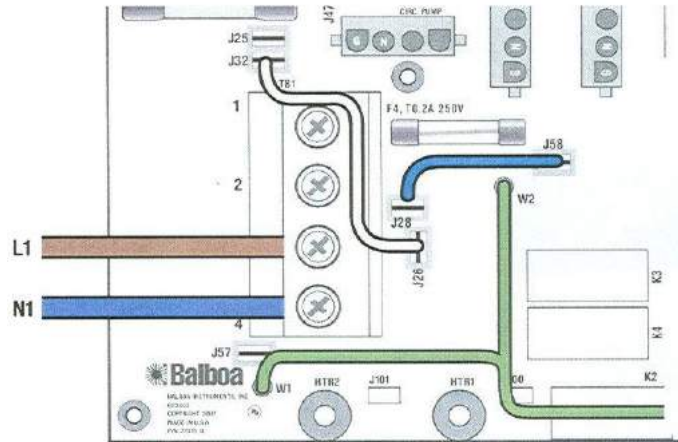
Figure 4. Single Phase Power – TN and TT Electrical Systems
