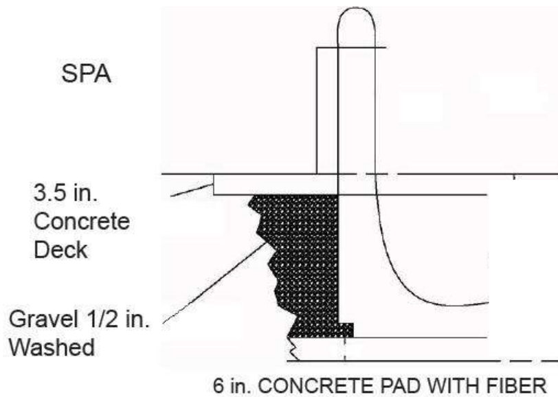
Figure 9. Excavation Cross Section
