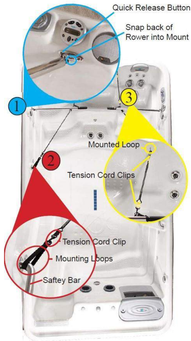
Figure 11. Rowing Equipment and Tension Cord Mount Locations
