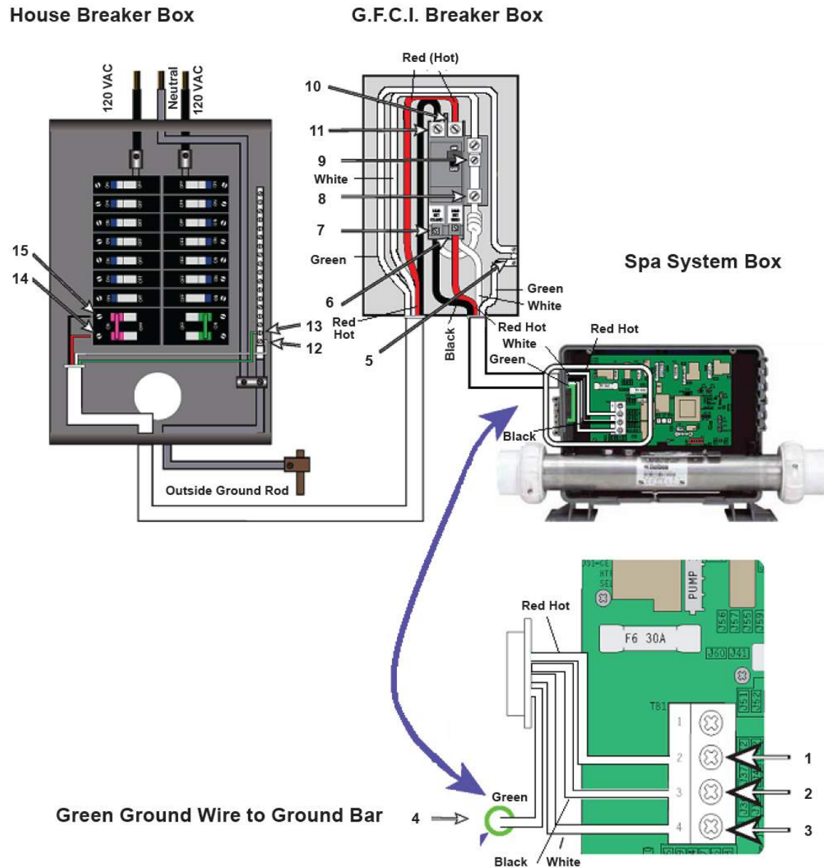
Figure 1. GFCI Wiring Schematic for 60 Hz Systems
